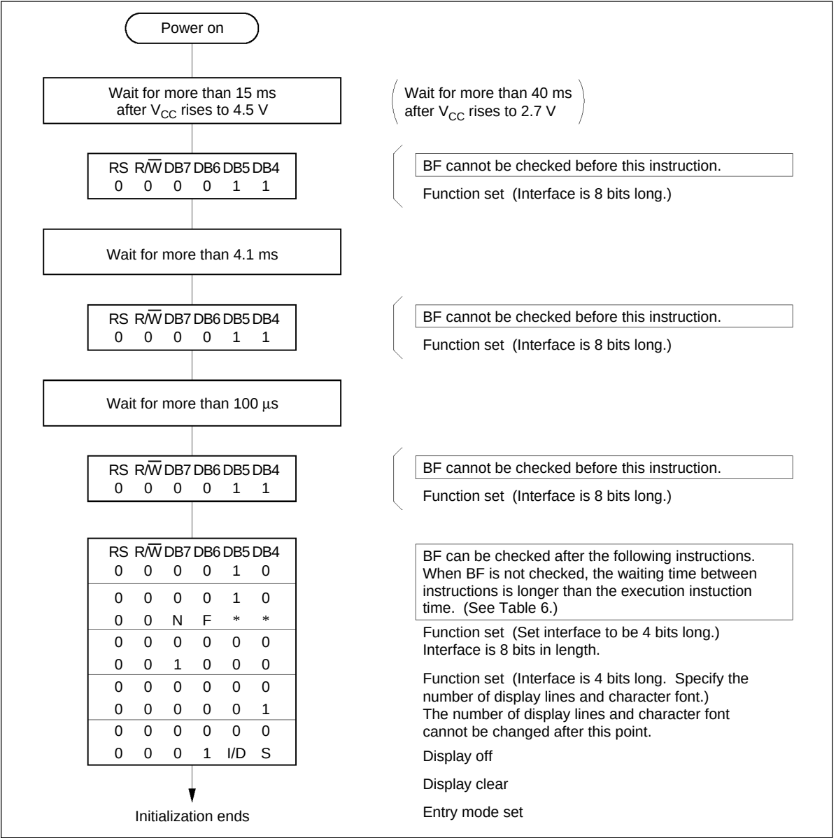
Figure 24 4-Bit Interface
